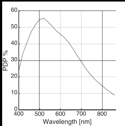
Photon detection probability.
