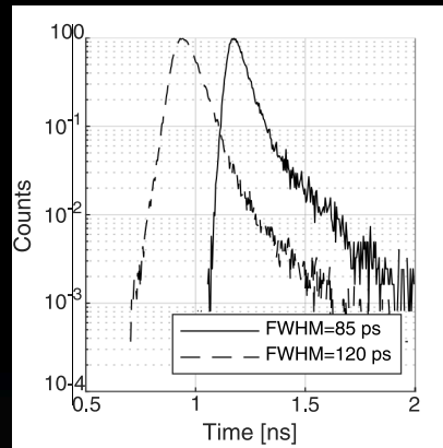
Excellent timing jitter with a FWHM of <150 ps for wavelengths between 510 and 785 nm.
