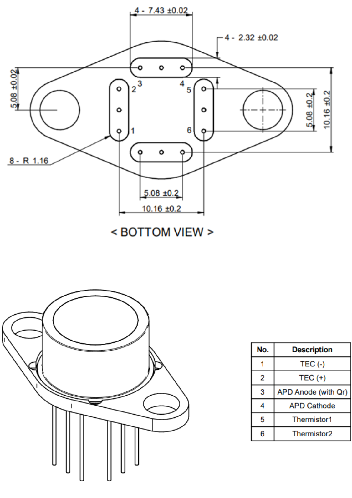
Figure 1. Mechanical Dimension and Standard PIN map
