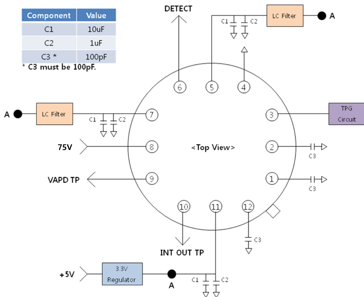
Figure 2. Application Circuit
