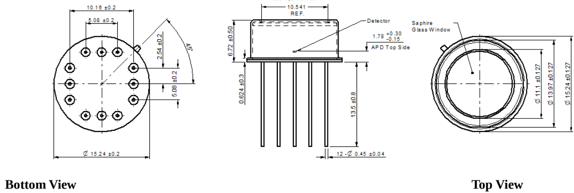
Figure 4. Mechanical Dimension
